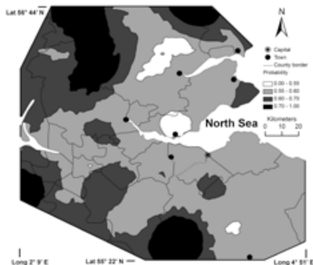
Fig. 1: Map example showing the application of disjunctive kriging for the variable Managed Maximum Flood Water Volume (m 3 , exceeding a threshold of 35 \times 10^4 m 3 ).
